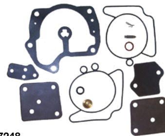
18-7248 KIT CARBURADOR Reemplaza: 437327, 439079, 439078, 435676, 435677, 435678, 435752
